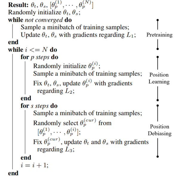
Algorithm 1: Alternating Adversarial Learning
